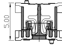
Mating Height Drawing
