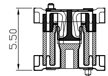
Mating Height Drawing
