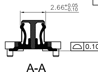
Mating Height Drawing
