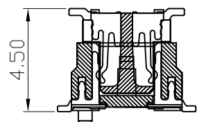
Mating Height Drawing
