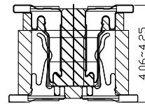
Mating Height Drawing
