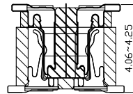
Mating Height Drawing
