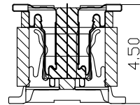
Mating Height Drawing
