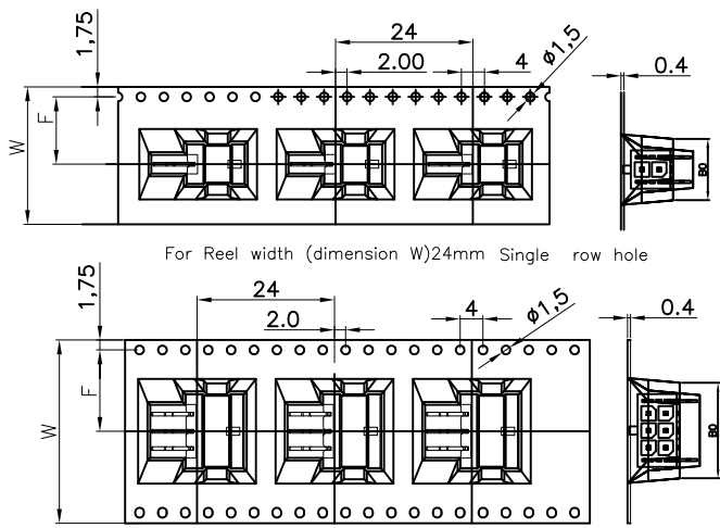
For Reel width (dimension W)24mm Single row hole
