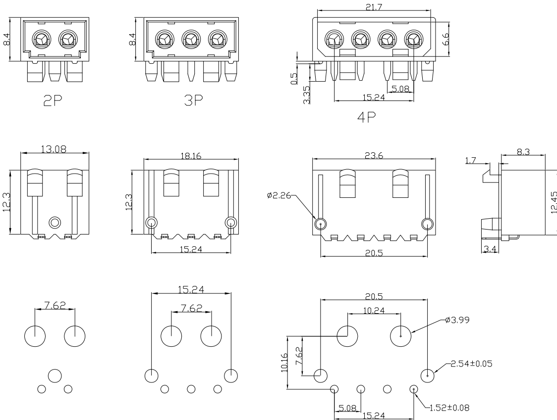
P. C. board hole dimensions
