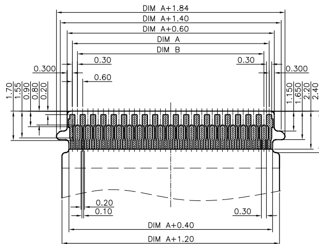
RECOMMENDED FPC/FFC DIMENSION
